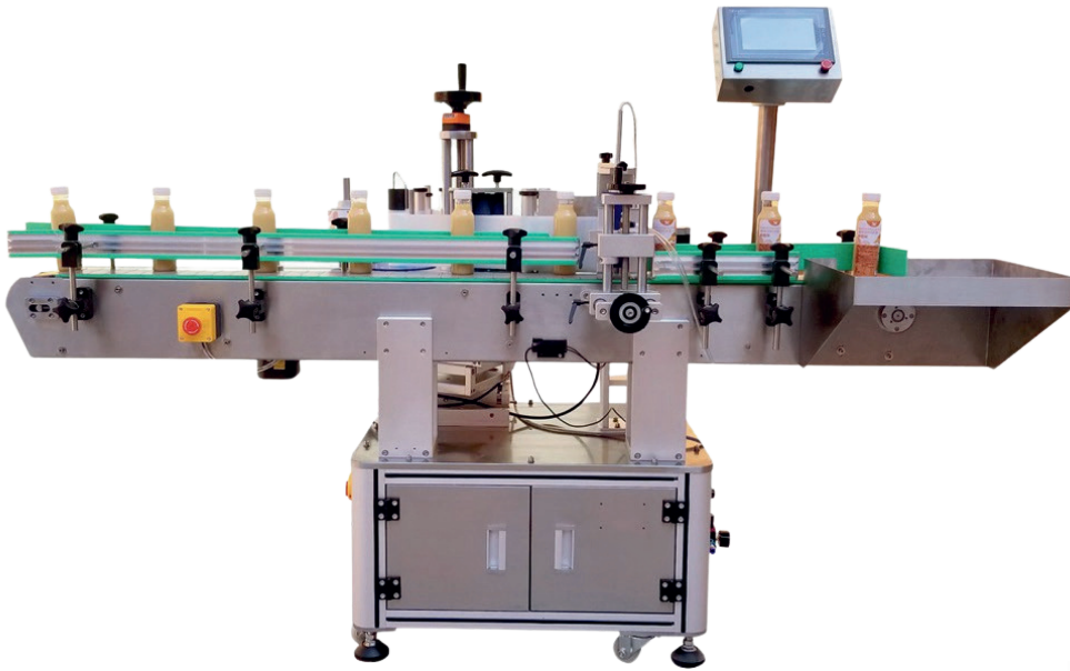
Automatic labeling machine for round format (1 label) in action:
