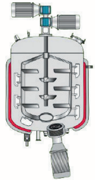
Double way mixing & internal circulation
